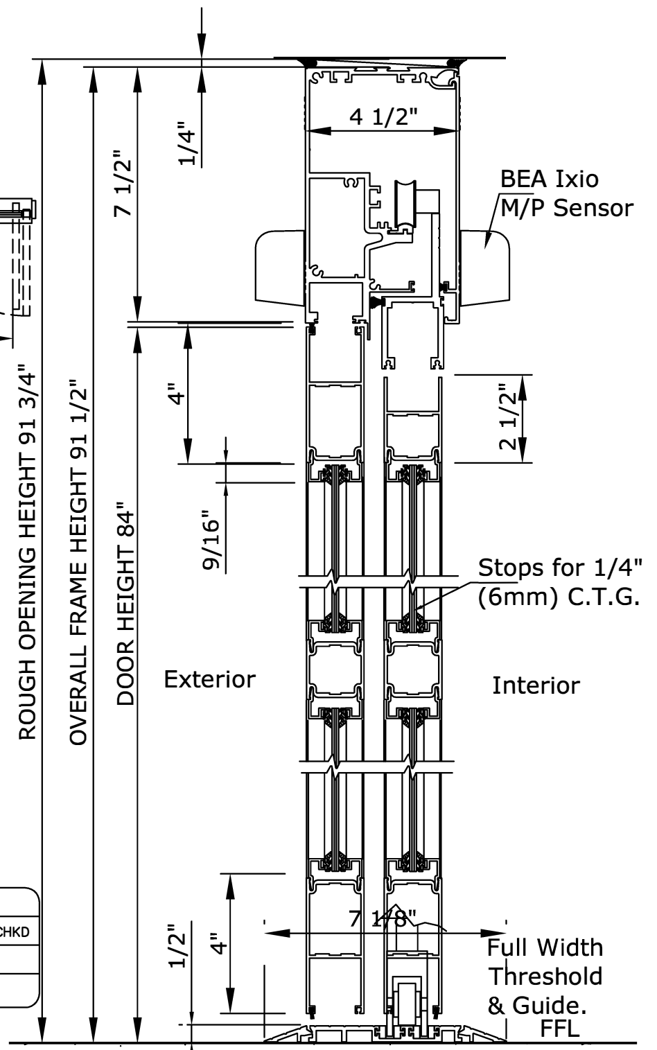
2 VERTICAL SECTION
