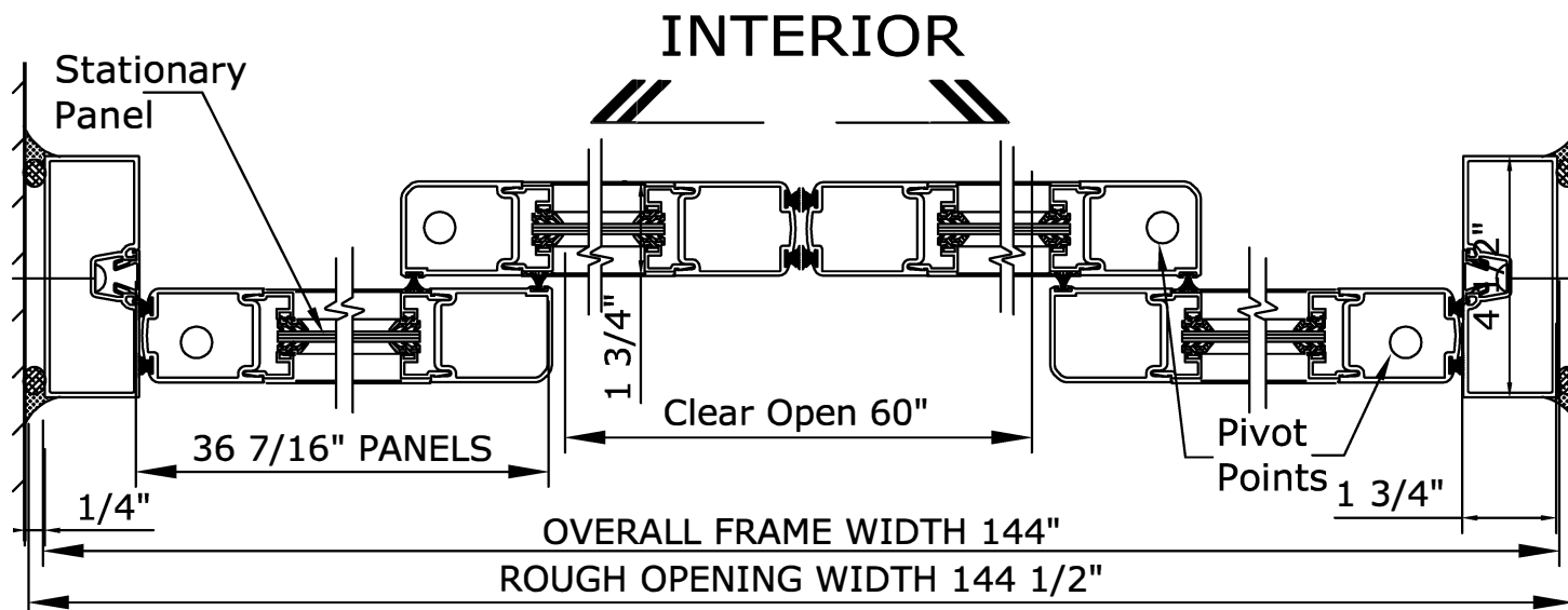
1 HORIZONTAL SECTION
