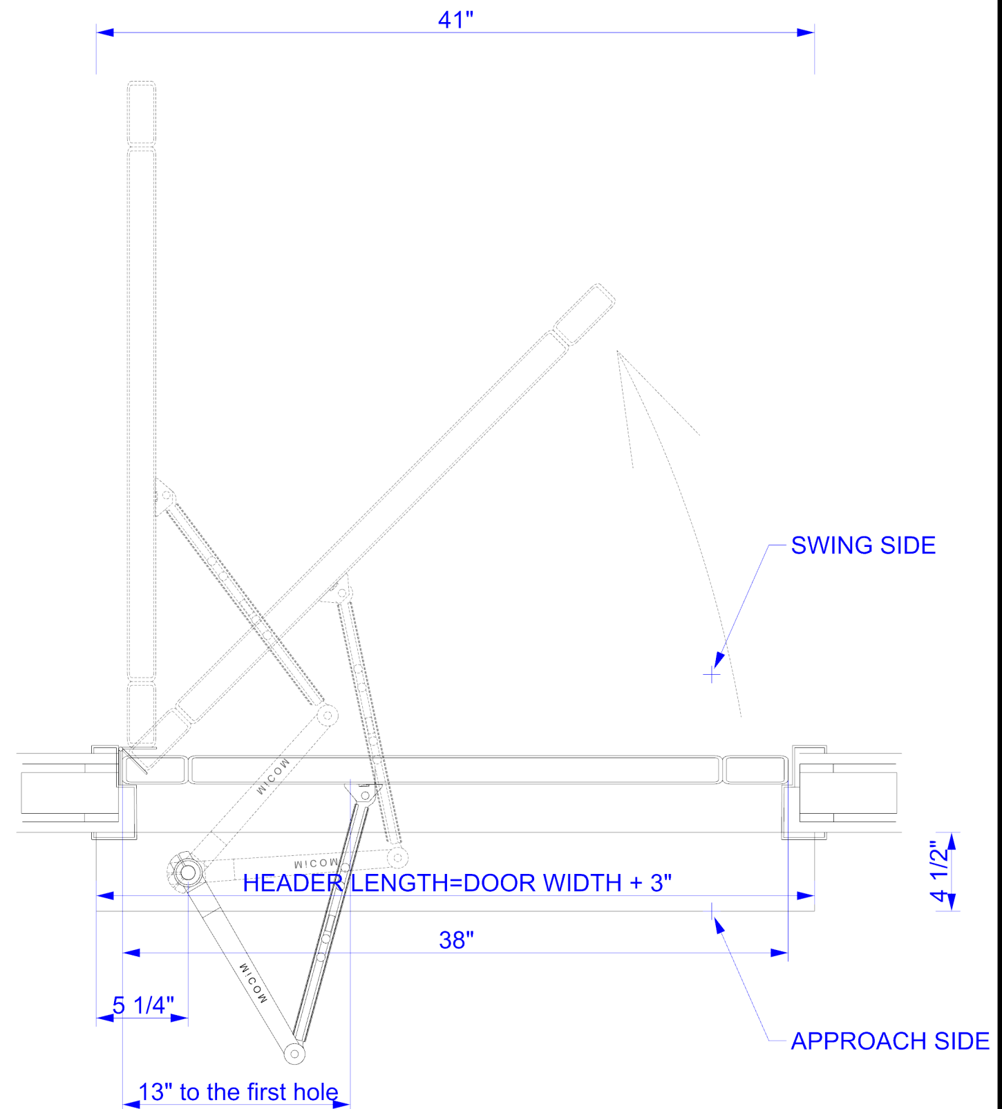
TOP VIEW
